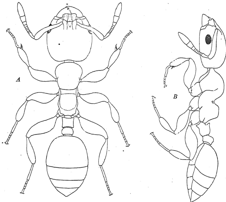
Fig. 1. Myrmecina panamana , new genus and new species. Worker. A, dorsal; B, lateral aspect.
