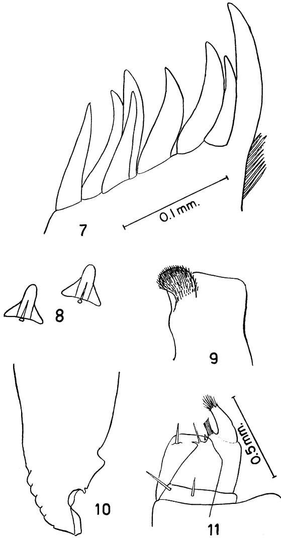
FIGS. 7-11. Phalloniscus avilensis (Van Name). 7. First maxilla. 8. Scale setae. 9. Second maxilla. 10. Extremity of the endopodite of the first male pleopods. 11. Maxilliped.
