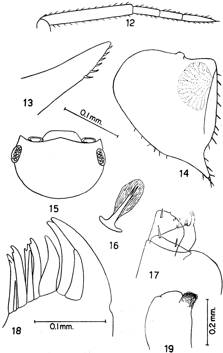
FIGS. 12-19. Balloniscus paraguayanus (Van Name). 12. Antenna. 13. Ex-tremity of the endopodite of the first male pleopods. 14. Exopodite of the first male pleopods. 15. Head from above. 16. Scale setae. 17. Maxilliped. 18. First maxilla. 19. Second maxilla.
