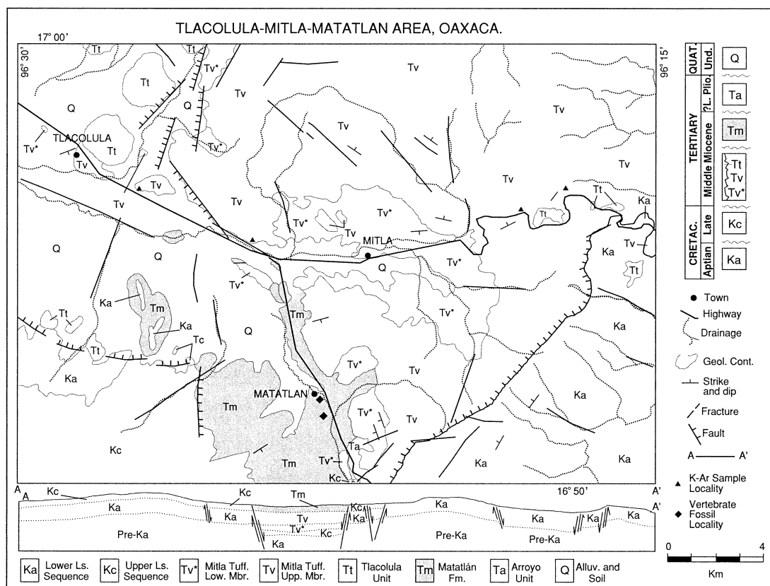
Fig. 13.4. Geologic map and generalized structural section of the Tlacolula-Mitla-Matatlán Area, Central Oaxaca.
