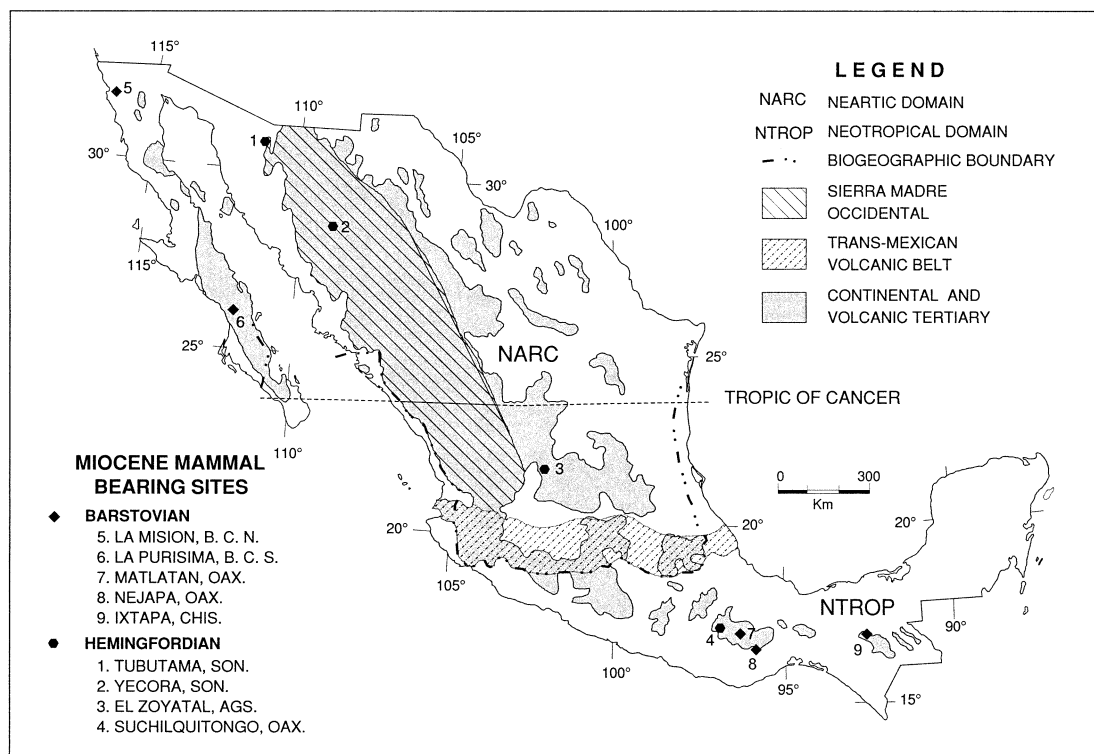
Fig. 13.1. Index map of Mexico showing location of areas mentioned in this study, the approximate extent of the continental sedimentary and volcanic Tertiary, two major geologic provinces, and present-day biogeographic domains.
