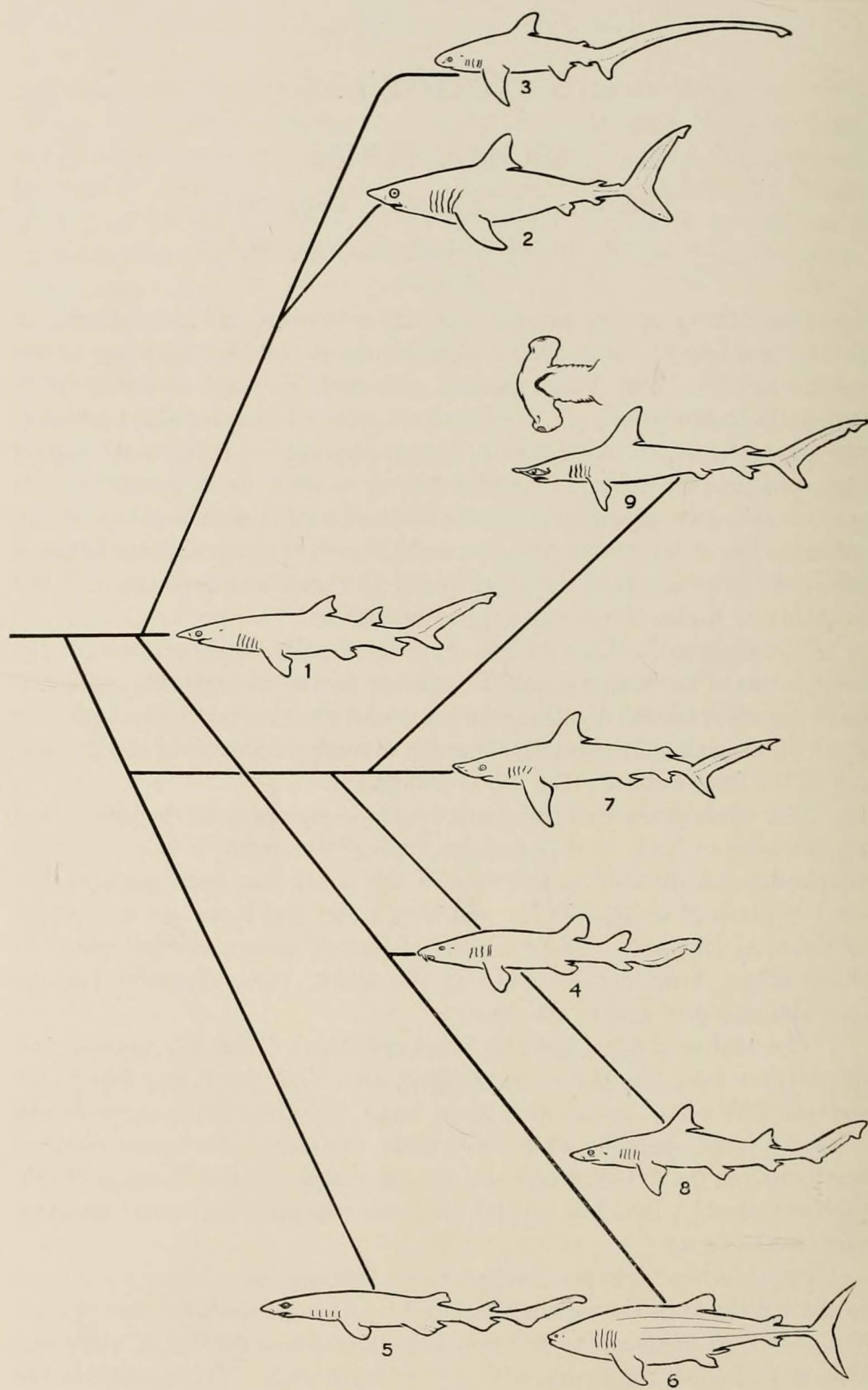
Fig. 3. Evolution of the Body Form of Sharks.
