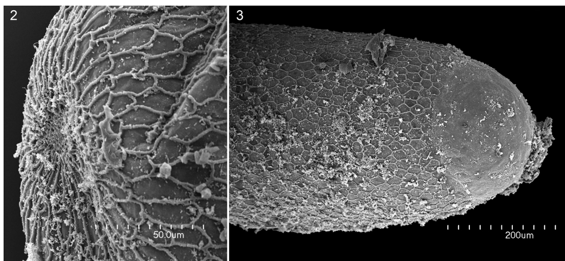
FIGURES 2, 3. SEM micrograph of 2, front and 3, posterior ends of egg of Plebeia “nan1” revealing geometric (mostly hexagonal) chorionic patterning at front and middle of egg and lack of patterning at rear (right).
