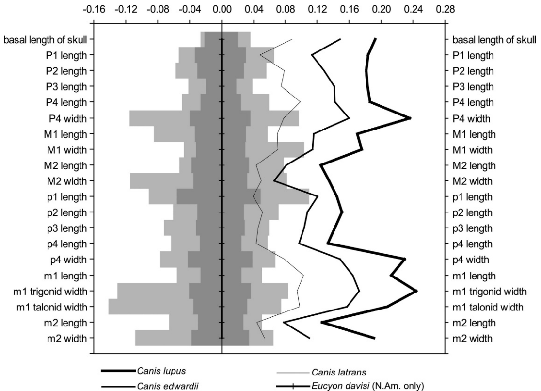
Fig. 51. Log-ratio diagram comparing the means of cheek tooth dimensions (appendix 3) of species of Canis against the North American sample of E. davisii (see appendix 3) as the reference. Canis lupus , western Canada, mean of 10 individuals, C. edwardii (n = 34), and C. latrans (n = 38) are shown. Gray bars extending from the mean of the standard are the observed ranges (light) and \pm 1 \sigma (dark).
