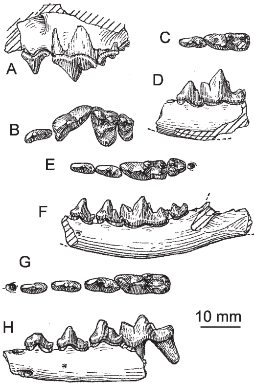
Fig. 23. A–D. Vulpes kermansis , early Hemphillian, California. A–B. Type maxillary fragment, LACM 55215. A. Lateral view, reversed. B. Occlusal view, reversed. C–D. Ramus, LACM 55216. C. Occlusal view. D. Lateral view. E–H. Vulpes sp. cf. V. velox , Irvingtonian, Nebraska. E–F. Ramus, UNSM 26163. E. Occlusal view, reversed. F. Lateral view, reversed. G–H. Ramus, F:AM 25516Z. G. Occlusal view. H. Lateral view.
