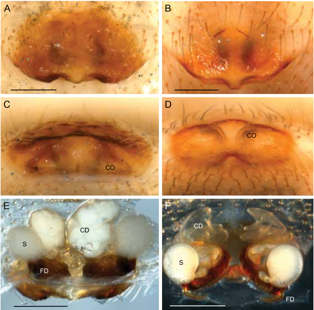
FIGURE 47. Taraira rufolineata (TEAU029; A , C , E ) and T. oculata (TEAU031; B , D , F ), epigyna. A , B . Ventral. C , D . Caudal. E , F . Dorsal digested. Scale bars: 0.2 mm.
