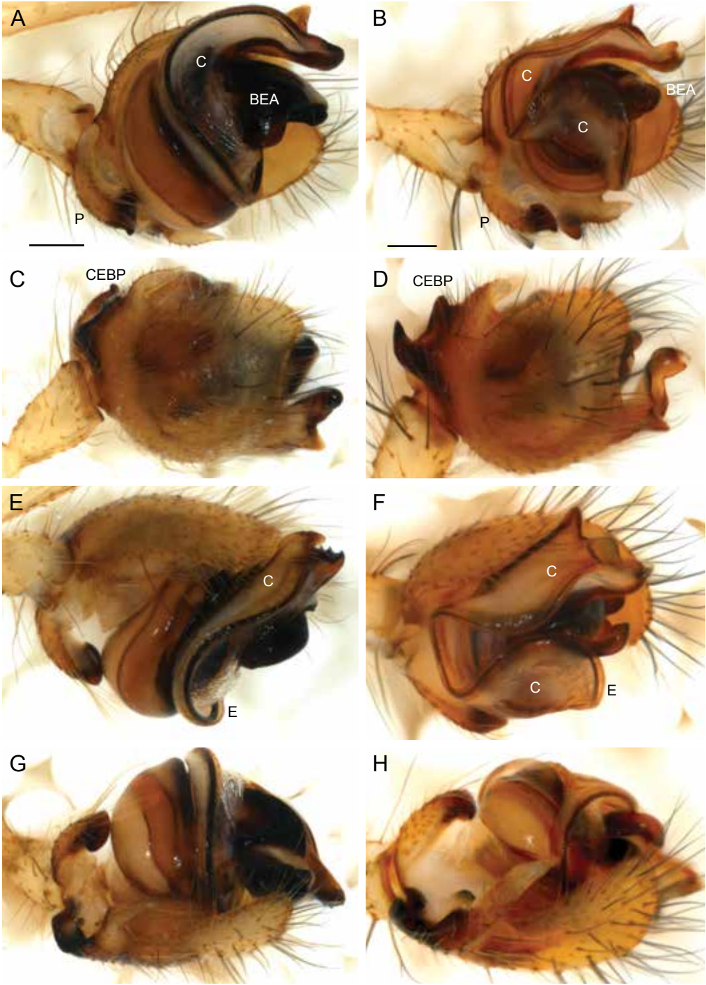
FIGURE 46. Tarairé rufolineata (TEAU030; A, C, E, G) and T. oculata (TEAU032; B, D, F, H), pedipalps. A, B. Ventral. C, D. Dorsal. E, F. Mesal. G, H. Ectal. Scale bars: 0.2 mm.
