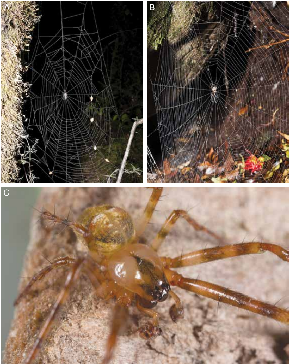
FIGURE 4. Taraira from New Zealand A. T. rufolineata (Urquhart, 1889) female web (DSC_7979). B. T. oculata female web (DSC_7919). C. T. oculata , adult male (G43A109). A: Arthur's Pass National Park, South Island; B, C: Fox Glacier, Westland Tai Poutini National Park, South Island (photos: G.H. except 4C, Gonzalo Giribet).
