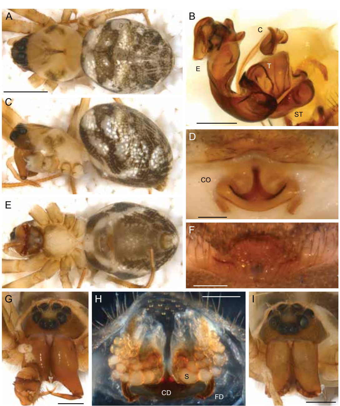
FIGURE 56. Iamarra multitheca (female: TEUA015, TEAU020; male: TEAU014, TEAU041). A. Female, dorsal habitus. B. Pedipalp, expanded. C. Female, lateral habitus. D. Epigynum, caudal. E. Female, ventral habitus. F. Epigynum, ventral. G. Male, frontal habitus. H. Epigynum, dorsal digested. I. Female, frontal habitus. Scale bars: A, C, E, 1.0 mm; B, 0.2 mm; D, F, H, 0.1 mm; G, I, 0.5 mm.
