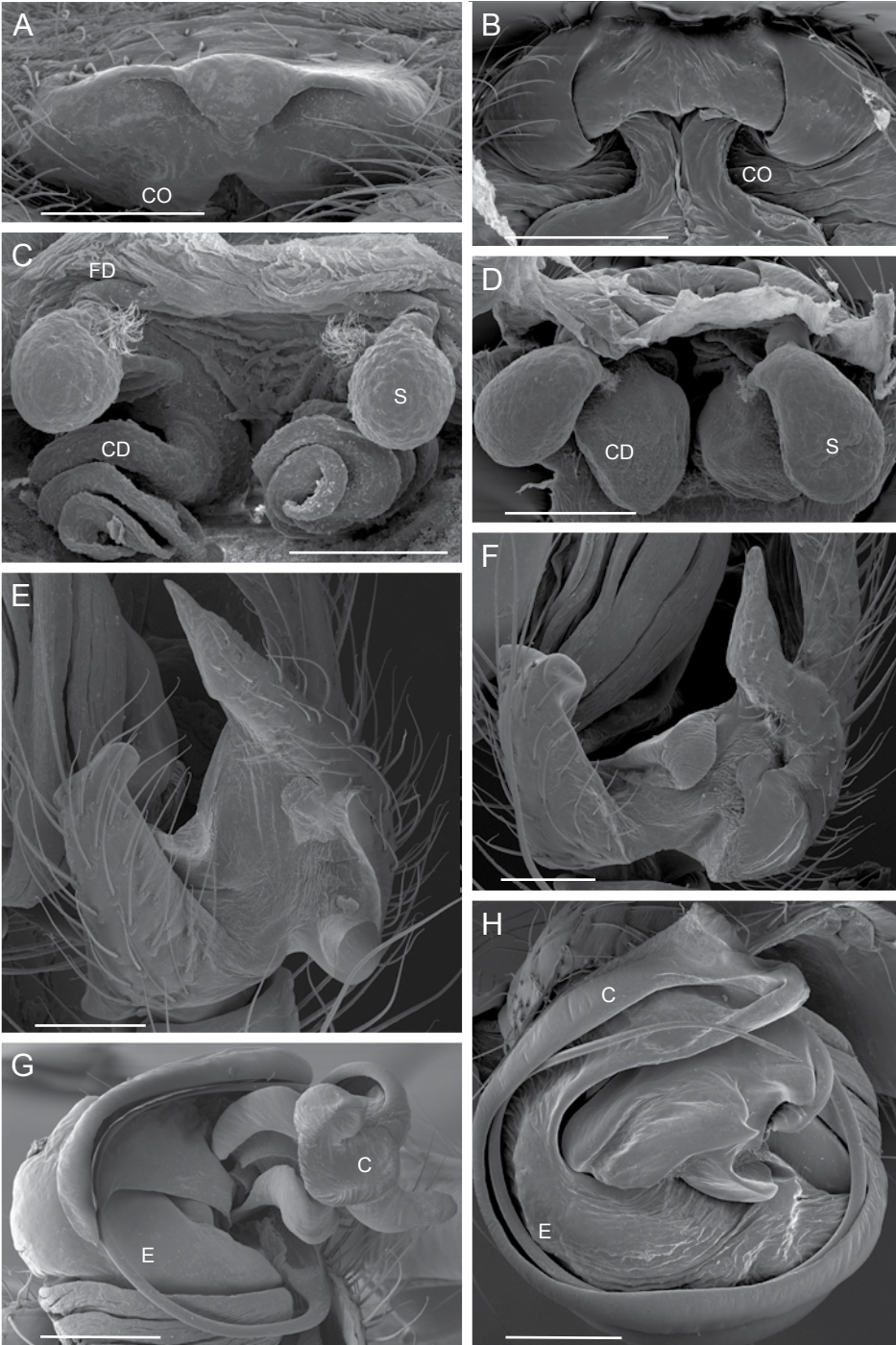
FIGURE 48. Taraira oculata (TEAU042; A, C, E, G) and T. rufolineata (female: TEAU043; male: TEAU046; B, D, F, H). A, B. Epigynum, caudal. C, D. Epigynum, dorsal. E, F. CEBP and CEMP, detail. G, H. Conductor and embolus apical detail. Scale bars: 0.2 mm.
