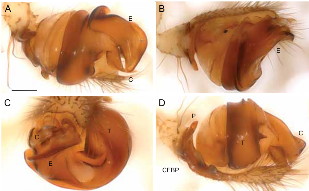
FIGURE 57. Tawhai multiteca pedipalp (TEAU014). A. Ventral. B. Mesal. C. Apical. D. Ectal. Scale bars: 0.2 mm.
