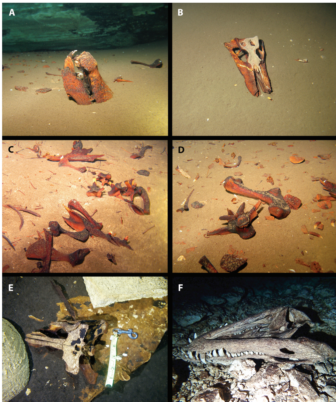
FIGURE 5. Underwater photographs of Late Quaternary fossils of the Cuban crocodile ( Crocodylus rhombifer ) from the Dominican Republic. A–E , Oleg’s Bat Cave: A . Skull and articulated mandible. B . Skull of second individual. C . Dentary and postcranial elements. Note very small slender bones of bats. D . Humerus and vertebra in center of photo, surrounded by osteoderms. E . Partial crocodile skull (scale in inches). F . Complete skull and articulated mandibles, from unnamed cave near Oleg’s Bat Cave. Specimen is “upside down” with mandibles on top. The skull and jaws in panel F were not collected.
