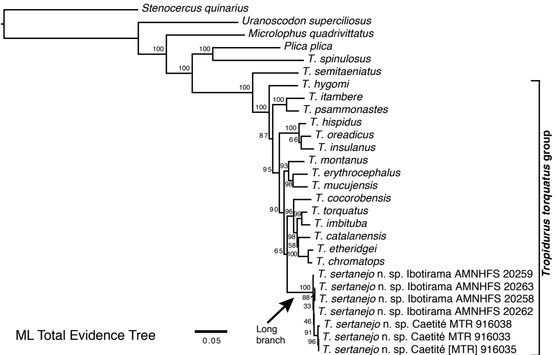
FIGURE 15. Maximum parsimony (upper) and maximum likelihood trees (lower) of Tropidurus on four mitochondrial (12S, 16S, CO1, Cyt b) and six nuclear loci (BACH1, kif24, NTF3, PRLR, PTPN, SNCAIP). Numbers associated to nodes refer to bootstrap values.
