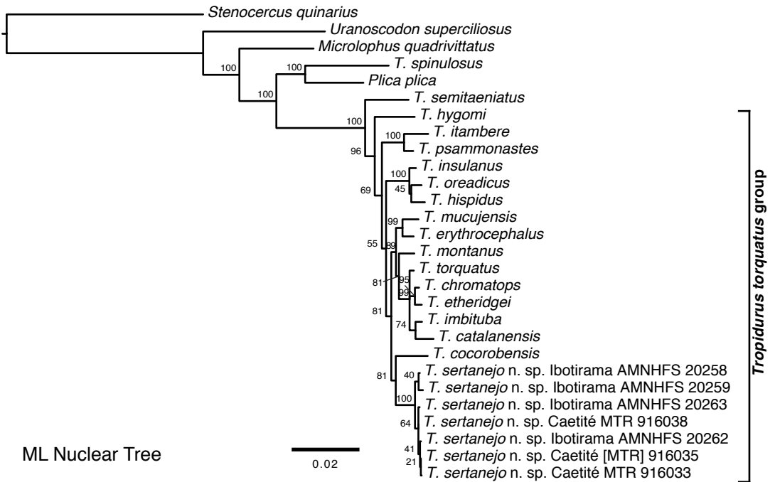
FIGURE 14. Maximum parsimony (upper) and maximum likelihood trees (lower) of Tropidurus based on four nuclear (BACH1, kif24, NTF3, PRLR, PTPN, SNCAIP) loci. Numbers associated to nodes refer to bootstrap values.
