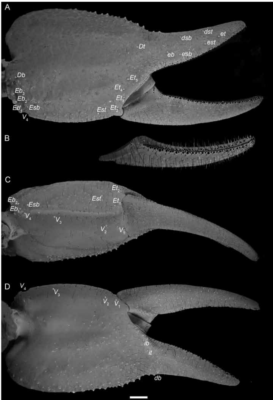
FIGURE 11. Kolotl magnus (Beutelspacher and López-Forment, 1991), n. comb., holotype ♀ (CNAN), dextral pedipalp chela, illustrating carinae and trichobothria. A. Retrodorsal aspect. B. Movable finger, dorsal aspect illustrating dentition. C. Ventral aspect. D. Proventral aspect. Scale bar = 1 mm. Abbreviations: Db , db , distal basal; dsb , distal subbasal; dst , distal subterminal; Dt , distal terminal; Eb , eb , external basal; Esb , esb , external subbasal; Est , est , external subterminal; Et , et , external terminal; ib , internal basal; it , internal terminal; V , ventral.
