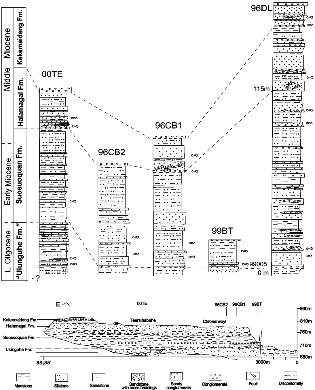
Fig. 21.3. Measured sections from the Tiersihabahe-Chibaerwoyi cliffs (TCC) in the northern Junggar Basin, showing the lithology, formation boundaries, occurrences of fossils, and thickness in meters. The sequence at the Tiersihabahe locality (00TE) is described in the text. Section 96DL is from the Duolebulejin area on the south bank of the Ulungur River (fig. 21.1), and other sections are drawn to the same scale.
