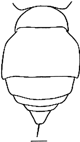
Figs. 43–48. Neotropical Polistinae. 43–44. Head in frontal view. 43. Protopolybia sedula (de Saussure). 44. Charterginus fulvus Fox. 45–46. Dorsal view. 45. Protopolybia sedula (de Saussure). 46. Charterginus fulvus Fox. 47. Polybia depressa (Ducke), metasoma in dorsal view. 48. Charterginus fulvus Fox, head and mesosoma in lateral view. All scale bars are 1.0 mm.
