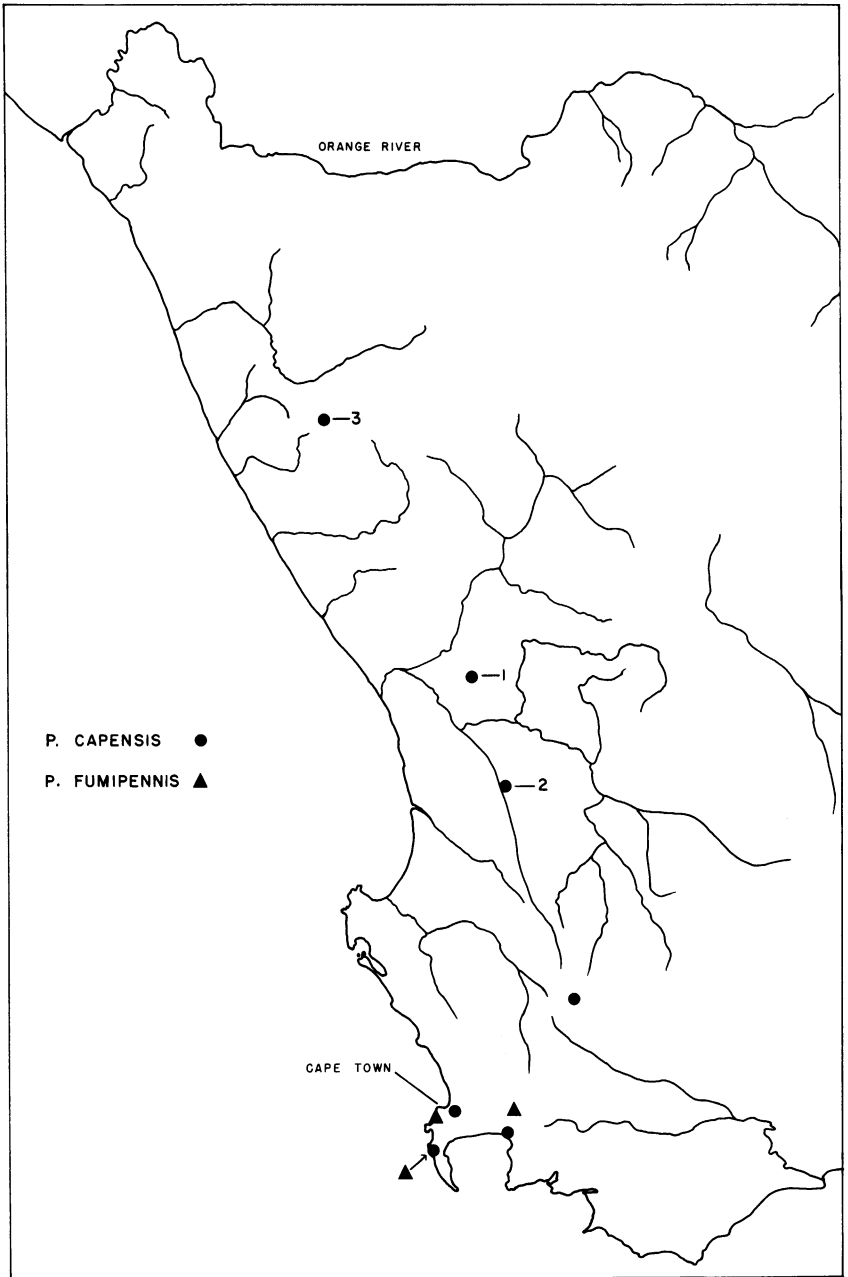
FIG. 1. Western Cape region of the Republic of South Africa, showing distribution of Pseudodichroa capensis and fumipennis .
