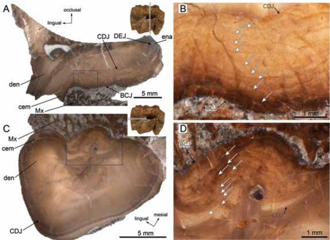
FIG 25. Dental histology of left M2 of Huayqueriana cf. H. cristata IANIGLA-PV 29. Coronal section: A , whole surface and B , detail of cementum layer (rectangle in A). Para-occlusal section: C , whole surface and D , detail of cementum layer (rectangle in C). Cementum rest lines indicated by white arrows. Abbreviations: BCJ , bone-cementum junction; CDJ , cementum-dentine junction; cem , cementum; DEJ , dentine-enamel junction; den , dentine; ena , enamel; Mx , maxilla.
