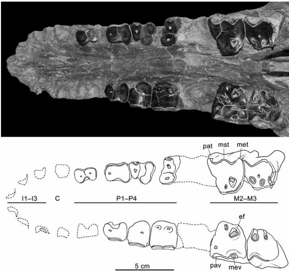
FIG. 24. Palate of Huayqueriana cf. H. cristata IANIGLA-PV 29, with detail of dentition in occlusal view. Abbreviations: C , canine (alveolus); ef , enamel fossette; I , incisor (alveolus); M , molar; met , metastyle; mev , metacone valley; mst , mesostyle; P , premolar; pat , parastyle; pav , paracone valley.
