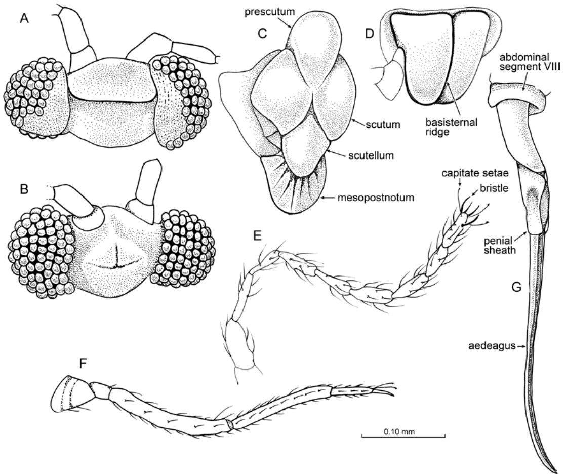
FIGURE 3. Details of Kozarius perpetuus , n. sp. (A) Dorsal head. (B) Ventral view of head. (C) Dorsal view of mesothorax. (D) Basisternum. (E) Antenna. (F) Leg. (G) Side view of penial sheath.
