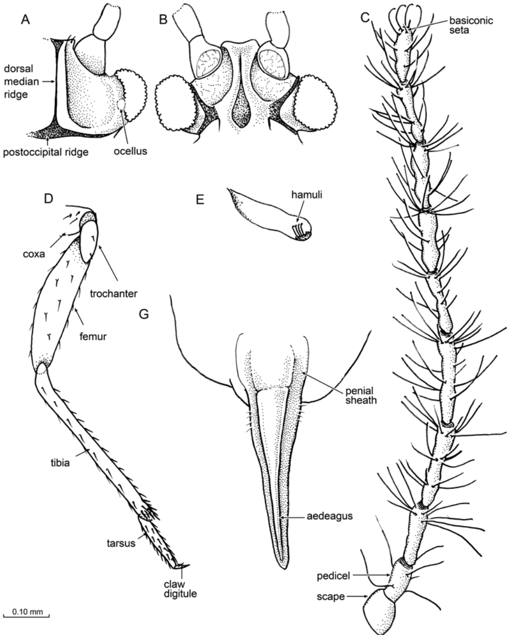
FIGURE 2. Details of Pseudoweitschatus audebertis , n. sp. (A) Dorsal view of head. (B) Ventral view of head. (C) Antenna. (D) Leg. (E) Hamulohaltere. (G) Ventral view of penial sheath.
