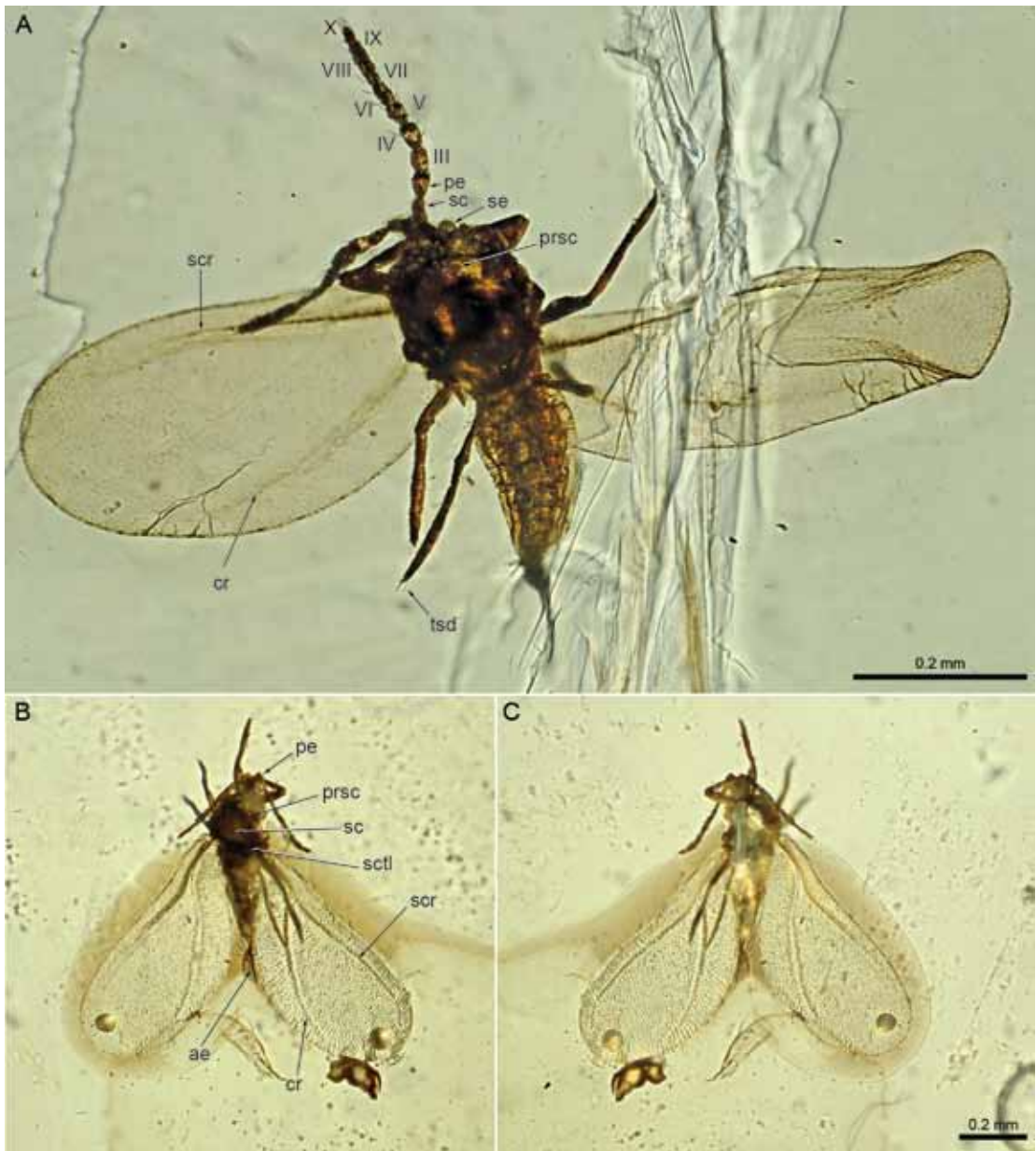
FIGURE 9. Photomicrographs of the new species of Apticoccus . (A) Dorsal surface of Apticoccus fortis , n. sp., holotype HAM-1669A. (B) Dorsal and (C) ventral surfaces of Apticoccus longitenuis , n. sp., holotype AD-20.
